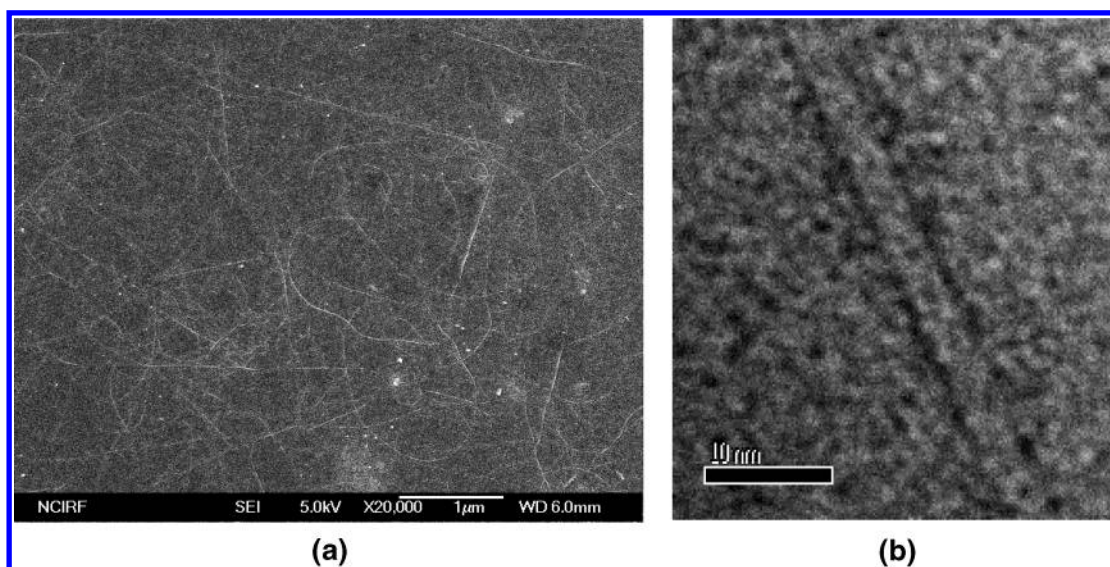
Figure 2. (a) Field emission scanning electron microscopy (FE-SEM) image of SWCNTs grown on binary array consisting of 3.3-nm iron oxide and 2.0-nm zirconia nanoparticles deposited on a \text{SiO}_2/\text{Si} wafer. (b) HRTEM image of SWCNT grown on a binary array consisting of 3.3-nm iron oxide and 2.0-nm zirconia nanoparticles.
