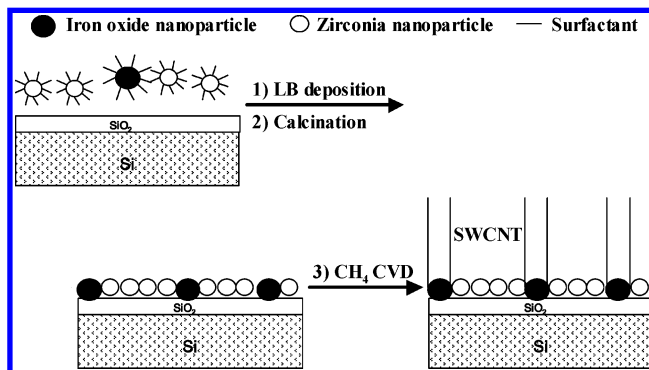
SCHEME 1: Schematic Representation of the Synthetic Procedure: (1) LB Deposition of Binary Nanoparticle Array, (2) Calcination to Remove Surfactant, (3) CH 4 CVD Process.
