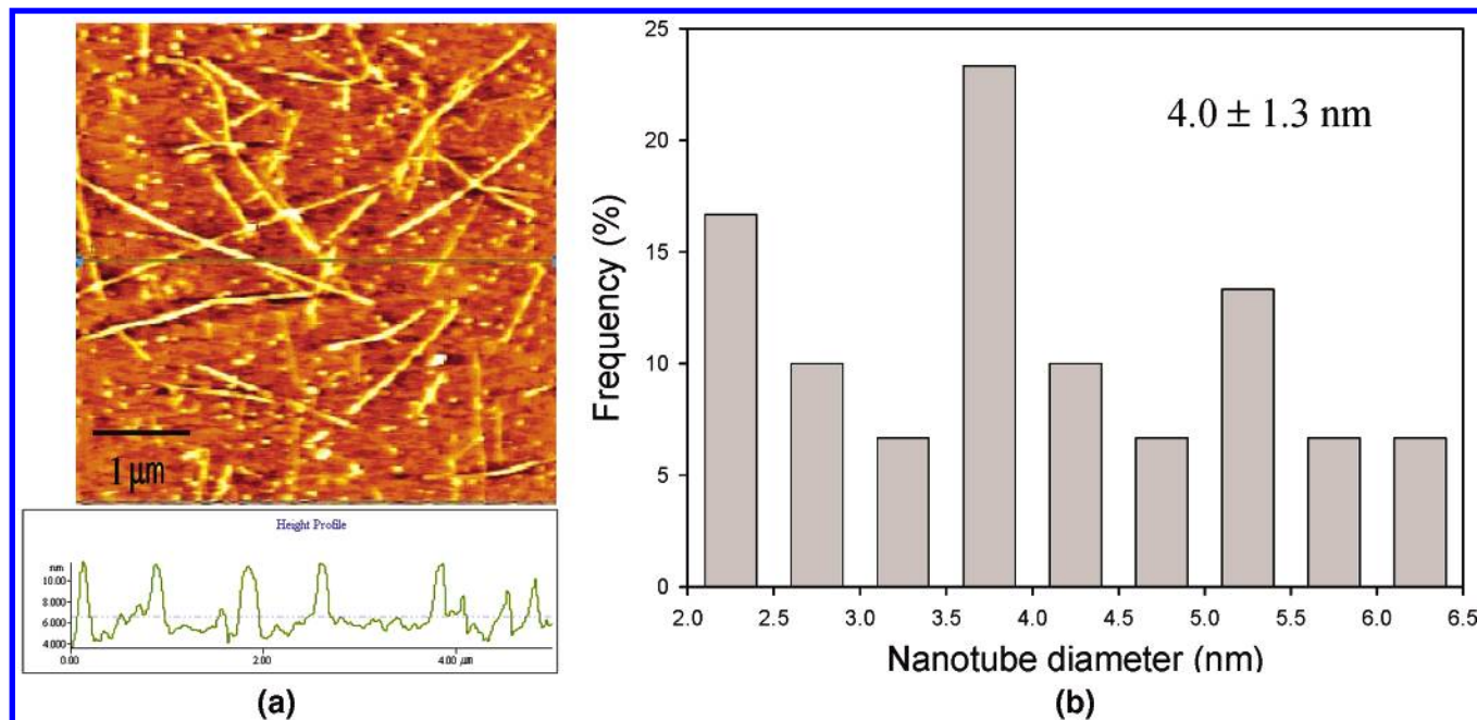
Figure 4. (a) AFM images of SWCNTs grown on 1.8-nm iron oxide deposited on a SiO 2 /Si wafer via spin coating. (b) Diameter distribution of SWCNTs grown on 1.8-nm iron oxide deposited on a SiO 2 /Si wafer via spin coating.
