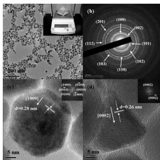
Figure 2. TEM micrographs of hexagonal pyramid-shaped ZnO nanocrystals. (a) Low-magnification TEM image. Inset: photograph of the obtained ZnO nanocrystals. (b) Electron diffraction (ED) pattern of ZnO nanocrystals. (c) HRTEM image showing the hexagon-shaped basal plane of ZnO nanocrystals. (d) HRTEM image showing the triangle-shaped side plane of ZnO nanocrystals. The insets are fast-Fourier transform (FFT) images of HRTEM images shown in (c) and (d).
