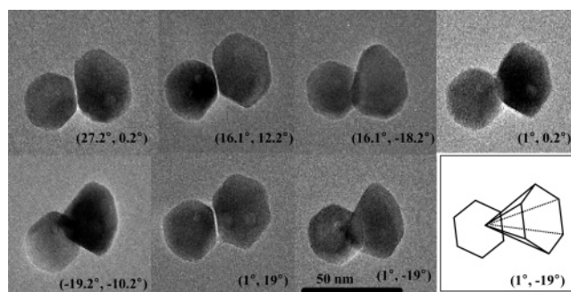
Figure 3. TEM images of hexagonal pyramid shaped ZnO nanocrystals at various tilted angles ( X^\circ , Y^\circ ) (left: hexagon shape, right: from hexagon shape to hexagonal pyramid image).
