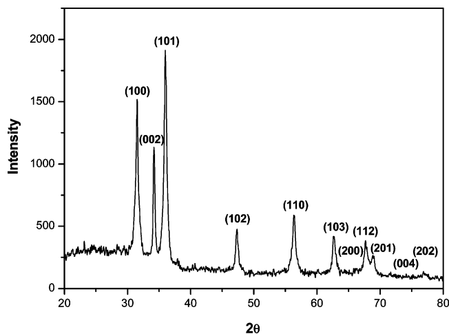
Figure 1. XRD pattern of hexagonal pyramid-shaped ZnO nanocrystals.
