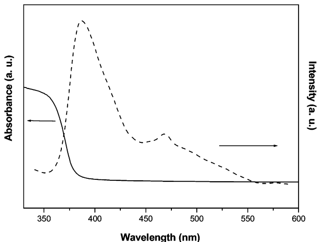
Figure 4. UV-vis. absorption and room-temperature PL spectra of the hexagonal pyramid-shaped ZnO nanocrystals.
