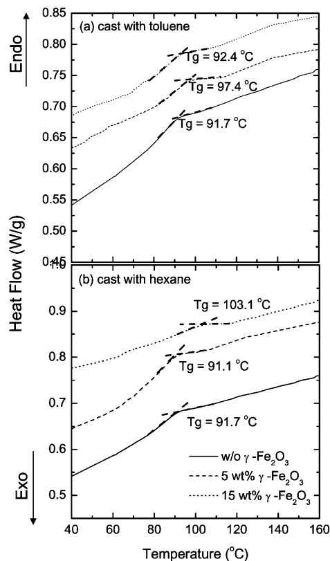
Figure 3. Differential scanning calorimetry traces of neat SI(39-12) and SI(39-12)/NP mixtures (with 5 and 15 wt % NPs) cast with (a) toluene and (b) hexane.
