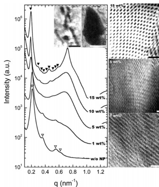
Figure 1. SAXS profiles for SI(39-12)/NP mixtures cast with toluene as a function of NP concentration. The lower trace ( \nabla ) of neat SI(39-12) represents the peaks with a ratio of 1:\sqrt{3}:\sqrt{7}:\sqrt{9} corresponding to the hex phase. The upper trace ( \blacktriangledown ) with 15 wt % NPs shows the well-developed bcc phase with a peak ratio of 1:\sqrt{2}:\sqrt{3}:\sqrt{4}... Cross-sectional TEM images of SI(39-12)/NP mixtures (1, 5, and 15 wt %) (PI domains are shown in black by the OsO 4 staining) are also shown. In particular, the block copolymer morphology with 15 wt % NPs is in good agreement with the bcc [001] direction. The TEM images in the inset of the SAXS profiles also show the magnetic strings with 3 wt % NPs and self-assembled NP lattices for 10 wt % NP loading. All scale bars are 100 nm.
