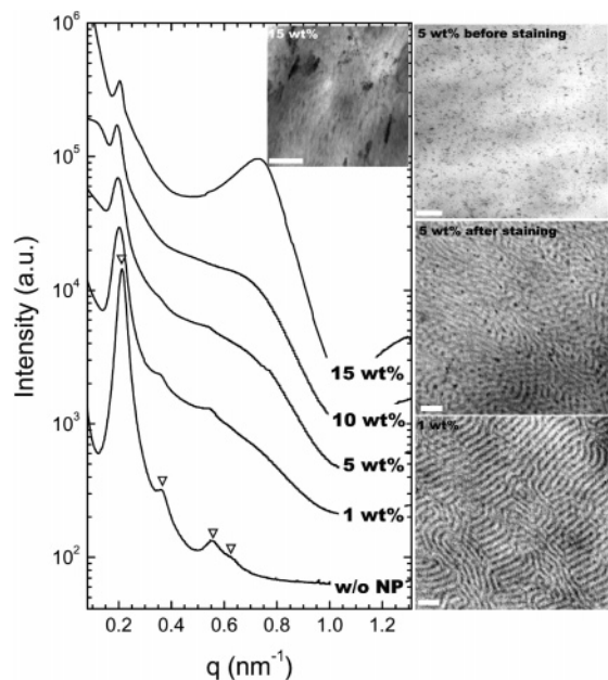
Figure 2. SAXS profiles for SI(39-12)/NP mixtures cast with hexane as a function of NP concentration. The lower trace ( \nabla ) of neat SI(39-12) again indicates the hex phase, and the block copolymer loses its long-range order as the NP concentration is increased. Cross-sectional TEM images of SI(39-12)/NP mixtures (1, 5, and 15 wt %) are also shown. Darker spots in each TEM micrograph represent the dispersed NPs of 7 nm diameter. The TEM image in the inset of the SAXS profiles shows the formation of NP strings coexisting with disordered block copolymer micelles. All scale bars are 100 nm.
